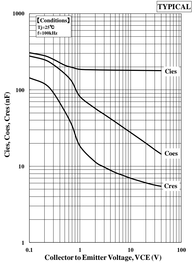
Capacitance vs. Collector to Emitter Voltage
