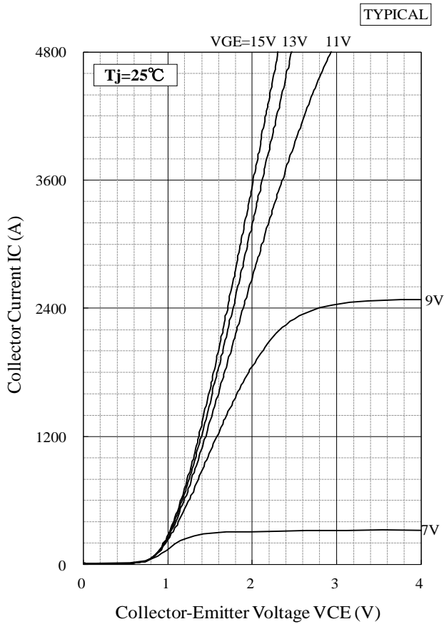
Collector Current vs. Collector to Emmitter Voltage
