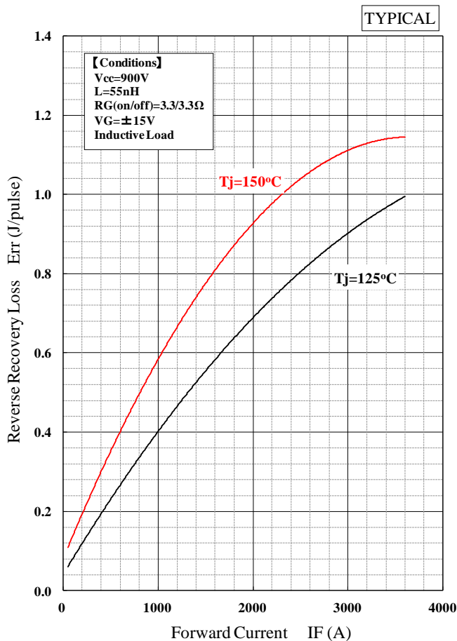
Reverse Recovery Loss vs. Forward Current
